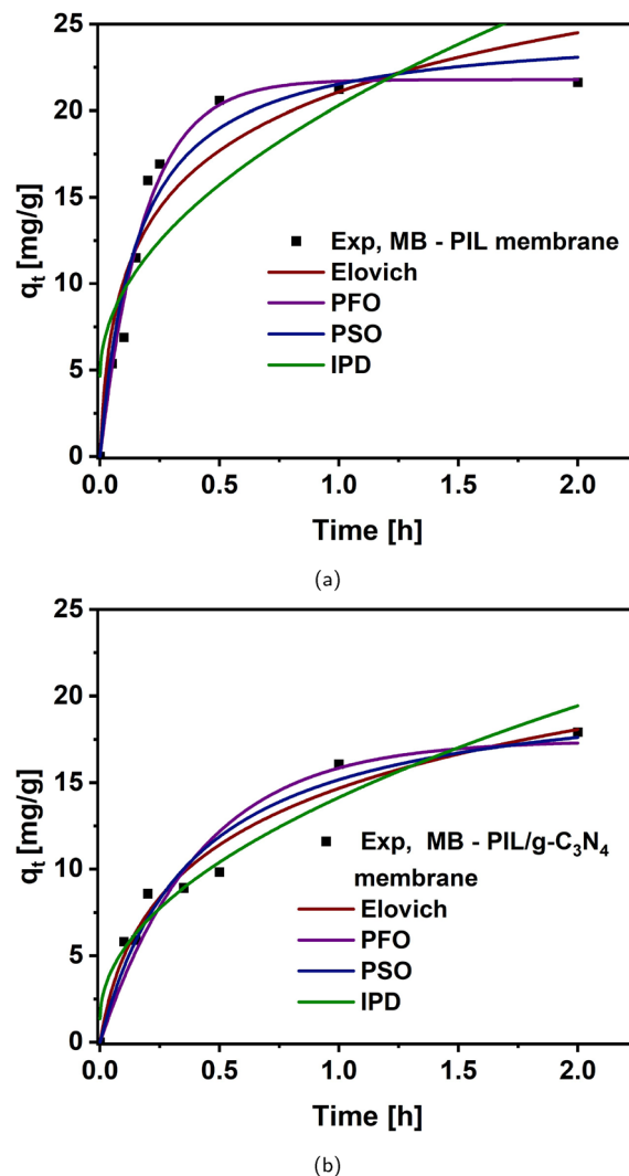
Fig. 7 Comparison of experimental and calculated adsorption capacity values ( q_t ) based on non-linear regression analysis of various kinetic models (pseudo-first-order (PFO), pseudo-second-order (PSO), Elovich, and intra-particle diffusion (IPD)) for adsorption of MB on (a) PIL, and (b) PIL/g-CN membranes.
