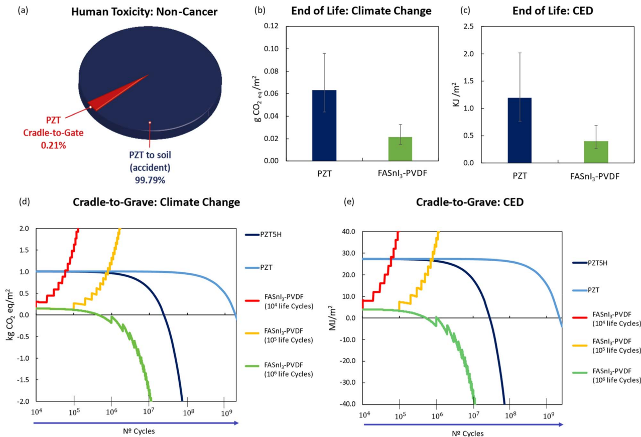
Fig. 8 (a) Comparison for Human toxicity: non-cancer impacts between cradle-to-gate impacts and accident soil releases; (b) end-of-life contribution to climate change for PZT and \text{FASnI}_3\text{-PVDF} ; (c) end-of-Life contribution to Cumulative Energy Demand (CED) for PZT and \text{FASnI}_3\text{-PVDF} ; (d) cradle-to-grave climate change impact as a function of the number of operational cycles; and (e) cradle-to-grave CED as a function of the number of operational cycles.
