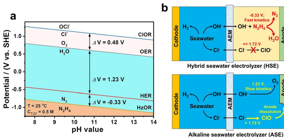
Fig. 9 (a) The Pourbaix diagram for OER, HER, HzOR, and ClOR in synthetic seawater containing 0.5 M Cl - at pH values ranging from 7 to 14. (b) Schematic illustration of hybrid seawater electrolysis design (HSE) (top) vs. alkaline seawater electrolysis design (ASE) (bottom). 81 Reproduced from ref. 81 with permission from Springer Nature, copyright 2021.
