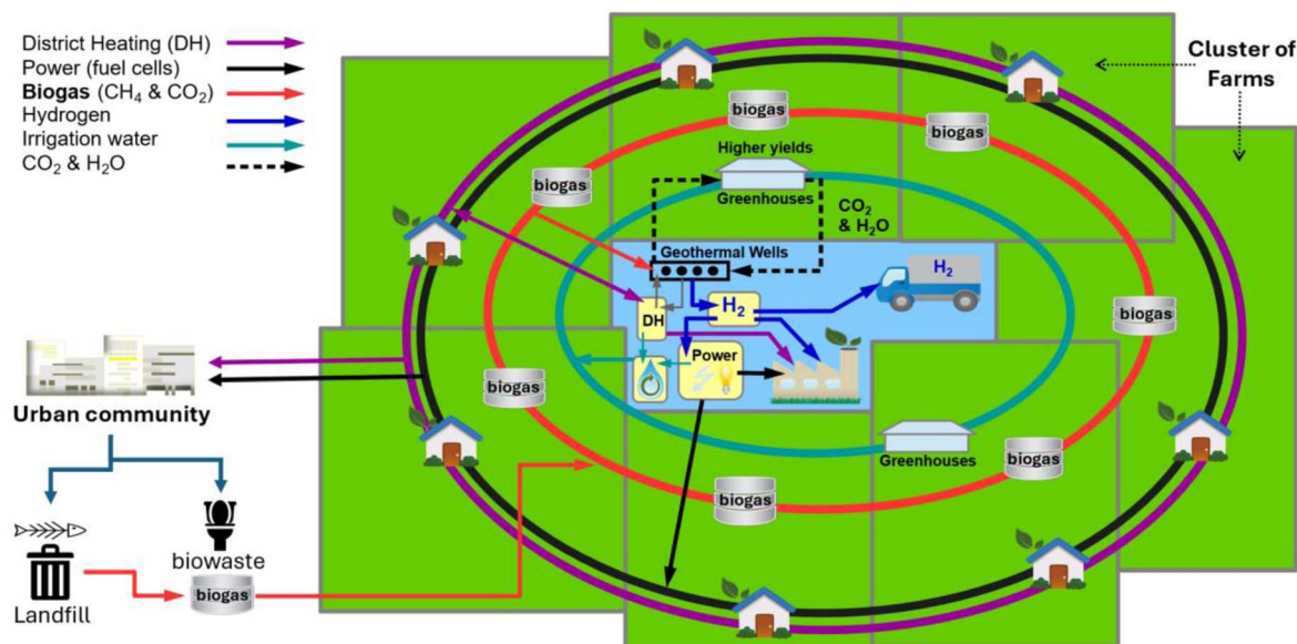
Fig. 2 An illustrated example of a cluster of farms with centrally located geothermal wells. The biogas labels refer to anaerobic digesters (AD) which create biogas and digester eco-fertilizers.
