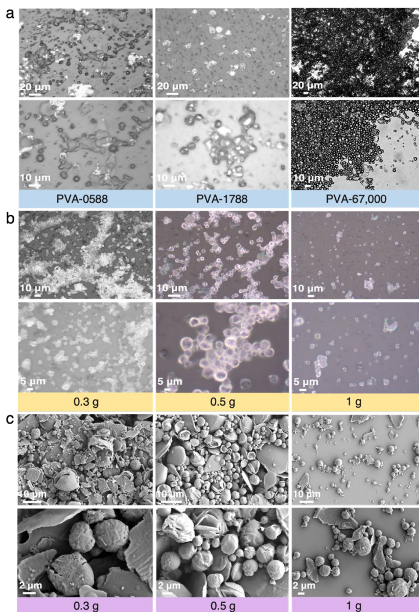
Figure 1. Optical images of PCMs microcapsules with different (a) emulsifier types, and (b) content of PVA-67,000. (c) SEM images of PCM microcapsules with different content of PVA-67,000.
