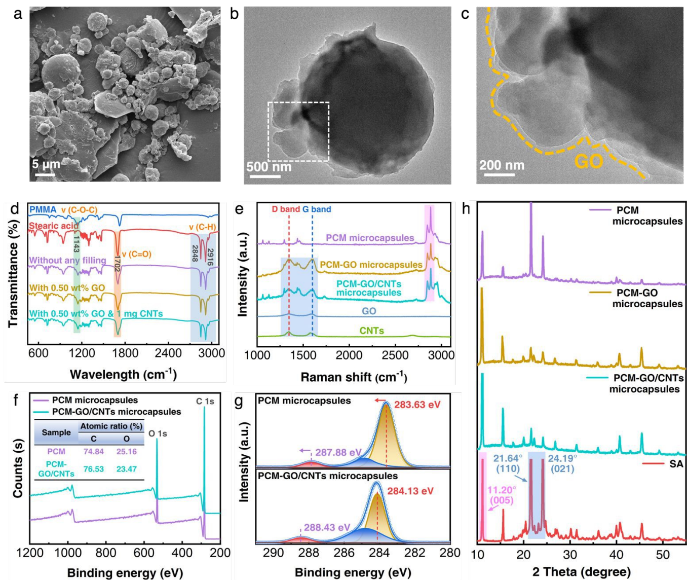
Figure 3. (a) SEM, (b) and (c) TEM images of PCM-GO/CNTs microcapsules. (d) FTIR spectra of (1) pure PMMA, (2) pure stearic acid, (3) 0.50 shell/core ratio of PCMs microcapsules, (4) 0.50 shell/core ratio with 0.5 wt% GO, and (5) 1.0 mg CNTs of PCMs-GO (0.5 wt%) microcapsules. (e) Raman scattering spectra of the PCM microcapsules, PCMs-GO microcapsules, PCMs-GO/CNTs microcapsules, GO and CNTs. (f) XPS spectra and (g) high-resolution C 1s spectra of PCM microcapsules and PCM-GO/CNTs microcapsules. (h) XRD patterns of (1) 0.50 shell/core ratio of PCMs microcapsules, (2) 0.50 shell/core ratio with 0.5 wt% GO, (3) 1.0 mg CNTs of PCMs-GO (0.5 wt%) microcapsules and (4) pure stearic acid.
