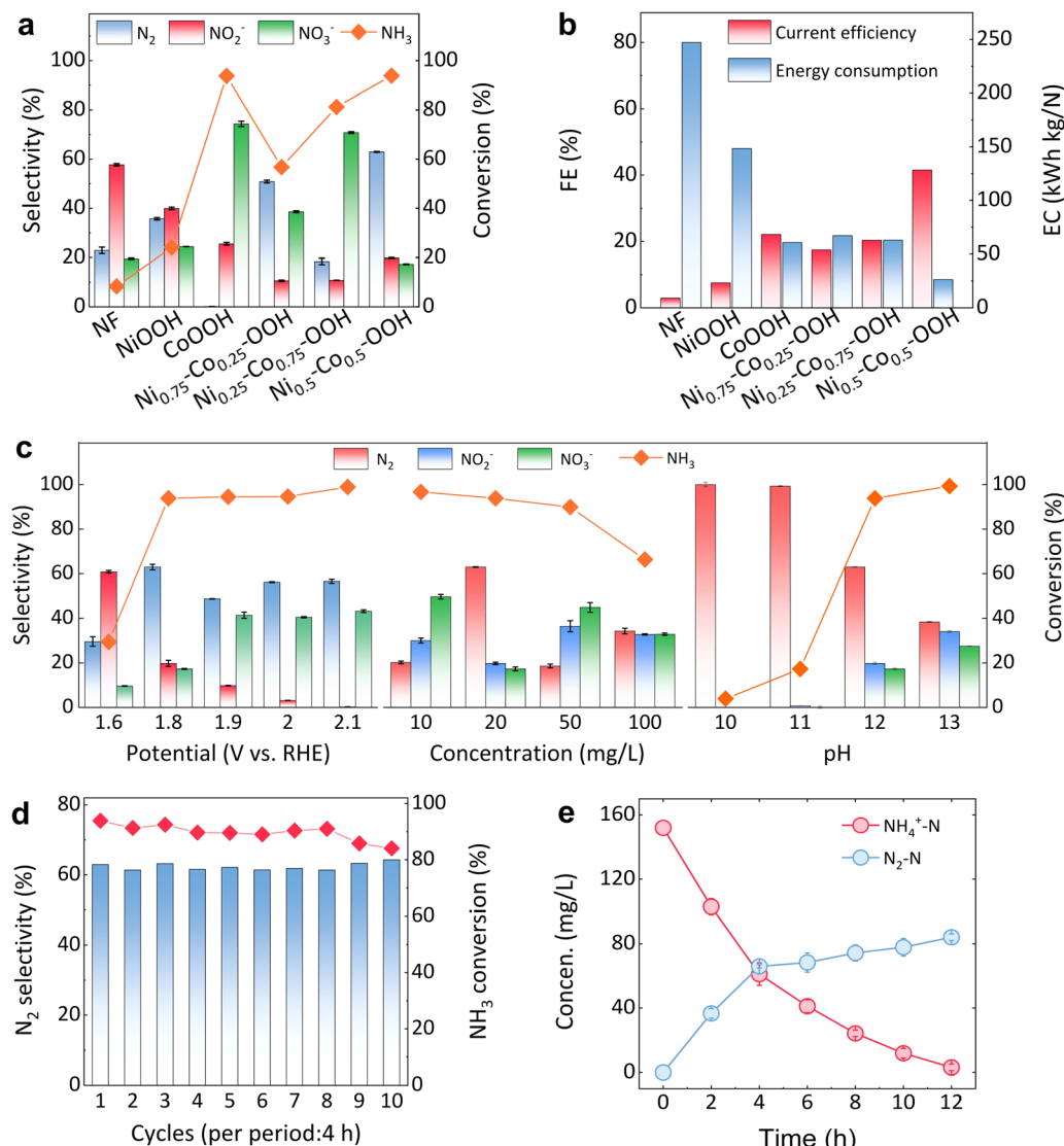
Fig. 3 (a) EAOR activity and product selectivity with different anodes ( E = 1.8 V, \text{pH} = 12 , 0.05 M \text{Na}_2\text{SO}_4 ); (b) Faradaic efficiency and energy consumption of the EAOR with different anodes ( E = 1.8 V, \text{pH} = 12 , 0.05 M \text{Na}_2\text{SO}_4 ); (c) EAOR activity and product selectivity of \text{Ni}_{0.5}\text{-Co}_{0.5}\text{-OOH} under different conditions; (d) ten cycles of \text{Ni}_{0.5}\text{-Co}_{0.5}\text{-OOH} ( E = 1.8 V, \text{pH} = 12 , 0.05 M \text{Na}_2\text{SO}_4 ); (e) EAOR activity of \text{Ni}_{0.5}\text{-Co}_{0.5}\text{-OOH} for practical wastewater ( E = 2.0 V, 0.05 M \text{Na}_2\text{SO}_4 ).
