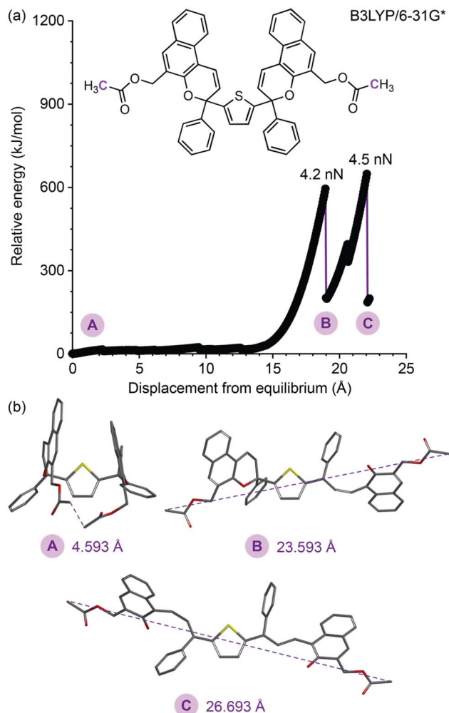
Fig. 1 (a) Density functional theory (DFT) calculations using the constrained geometries simulate external force (CoGEF) method performed on a truncated model of the 3H-bis-naphthopyran mechanophore predict the expected ring-opening reactions to generate mono-merocyanine and bis-merocyanine products. Calculations were performed at the B3LYP/6-31G* level of theory. (b) The corresponding computed structures of the truncated molecule at various points of elongation are shown along with the associated constraint distance between the terminal carbon atoms. Data for the (R,S) diastereomer shown (see the SI for additional information).
