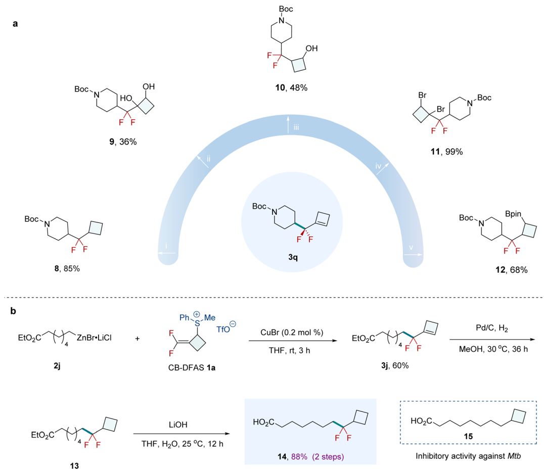
Scheme 5 Transformations of the 3q and synthesis of complex analogues. (i) Pd/C (5 mol%), H 2 , THF, 30 °C, 8 h. (ii) K 2 O 2 (OH) 4 (5 mol%), NMO (2.0 equiv.), acetone, H 2 O, rt, 20 h (iii) BH 3 THF (1.5 equiv.), THF, 0 °C, 2 h; (2) NaOH (14.0 equiv., 2 N), H 2 O 2 (16.0 equiv., 30% wt in water), rt, 2 h. (iv) CCl 4 (0.3 mL), Br 2 (1.5 equiv.), 0 °C, 2 h; (v) Ir 2 Cl 2 (COD) 2 (2.5 mol%), DPPE (5 mol%), DCM, HBpin (1.5 equiv.), –20 °C to rt, 20 h.
