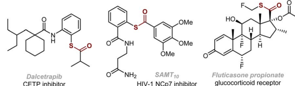
(b) Traditional methods for thioesters formation
