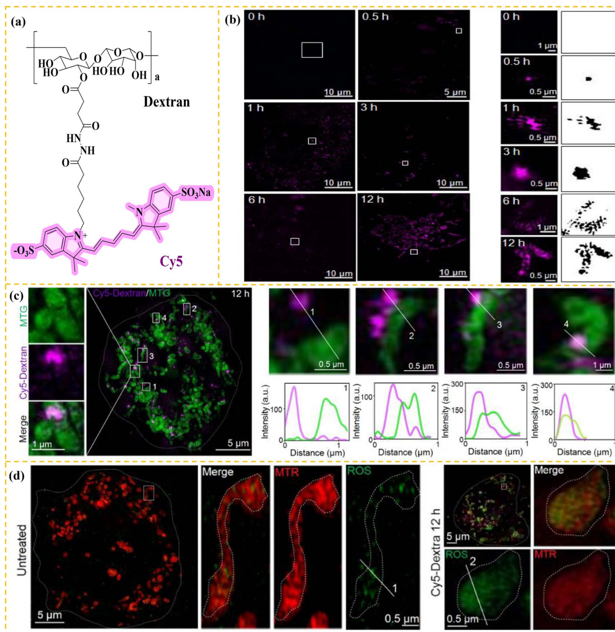
Fig. 54 (a) Chemical structure of probe Cy5-Dextran . (b) SIM imaging of the Cy5-Dextran probe targeting organelles in HeLa cells at different time periods. (c) SIM imaging of HeLa cell probe Cy5-Dextran in contact with mitochondria and mitochondrial fragmentation. (d) SIM imaging of the Cy5-Dextran probe and ROS commercial green probe for monitoring ROS levels in HeLa cells. Reprinted with permission from Elsevier, copyright 2022, as cited in ref. 132.
