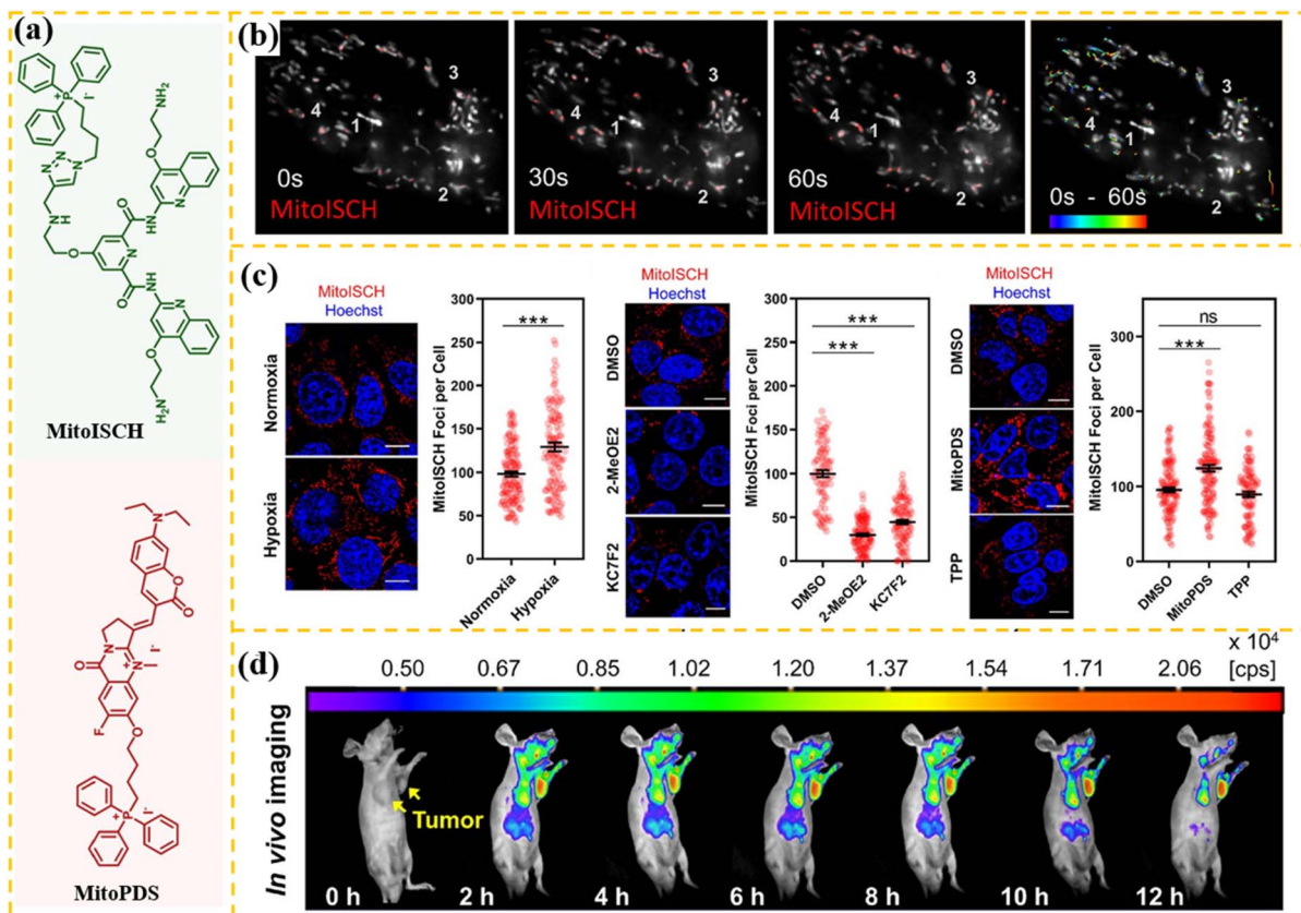
Fig. 15 (a) Chemical structures of the mtDNA G4-specific fluorescent probe MitoISCH and the mitochondria-targeted G4 ligand, MitoPDS . (b) SIM imaging of mtDNA G4 kinetics of probe MitoISCH in living cells. (c) Imaging of mtDNA G4 folding to glycolysis in HepG2 cells under hypoxic stimulation. (d) Imaging of probe MitoISCH in glycolysis in hormonal nude mice. Reprinted with permission from the American Chemical Society, copyright 2021, as cited in ref. 65.
