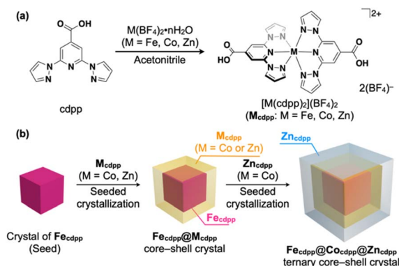
Fig. 1 (a) Synthetic scheme of \text{M}_{\text{cdpp}} ( M = \text{Fe}, \text{Co}, \text{Zn} ). cdpp: 4-carboxy-2,6-di(pyrazol-1-yl)pyridine. (b) Schematic illustration of core-shell crystals of \text{M}_{\text{cdpp}} using a seeded crystal growth method.
