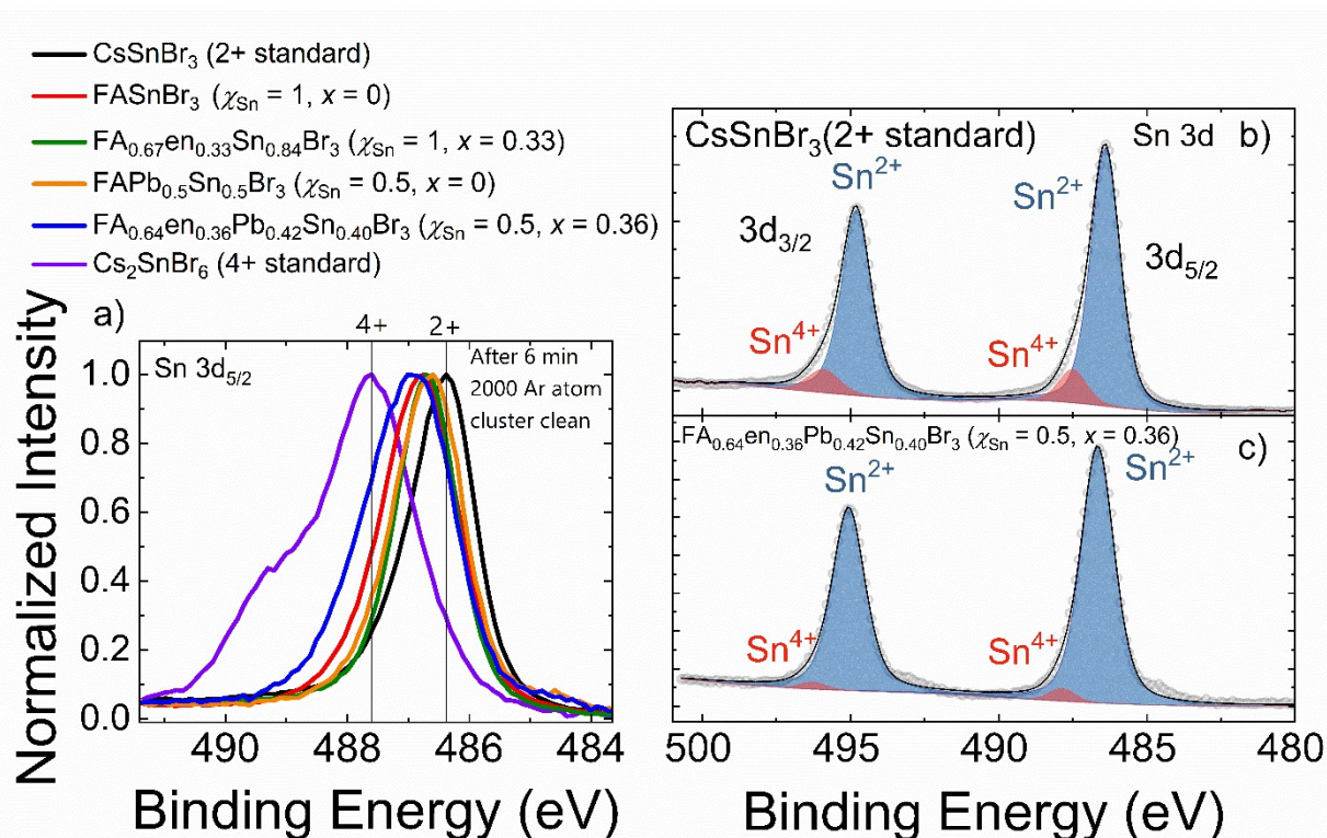
Figure 3. a) Sn 3d 5/2 spectrum of 2 standards (CsSnBr 3 and Cs 2 SnBr 6 ) and selected samples. The samples include a hMHP (FA 0.67 en 0.33 Sn 0.84 Br 3 ( \chi_{\text{Sn}} = 1 , x = 0.33 )), a mixed Pb/Sn (FAPb 0.5 Sn 0.5 Br 3 ( \chi_{\text{Sn}} = 0.5 , x = 0 )) and both hMHP and Pb/Sn mixed sample (FA 0.64 en 0.36 Pb 0.42 Sn 0.40 Br 3 ( \chi_{\text{Sn}} = 0.5 , x = 0.36 )). All samples have a similar FWHM and peak position as the FASnBr 3 . All the samples are mainly Sn 2+ with minor Sn 4+ components. b) Fitted Sn 3d spectra for the 2+ standard showing a small (11%) Sn 4+ contribution compared to sample c) FA 0.64 en 0.36 Pb 0.42 Sn 0.40 Br 3 ( \chi_{\text{Sn}} = 0.5 , x = 0.36 ), which showed only 4%.
