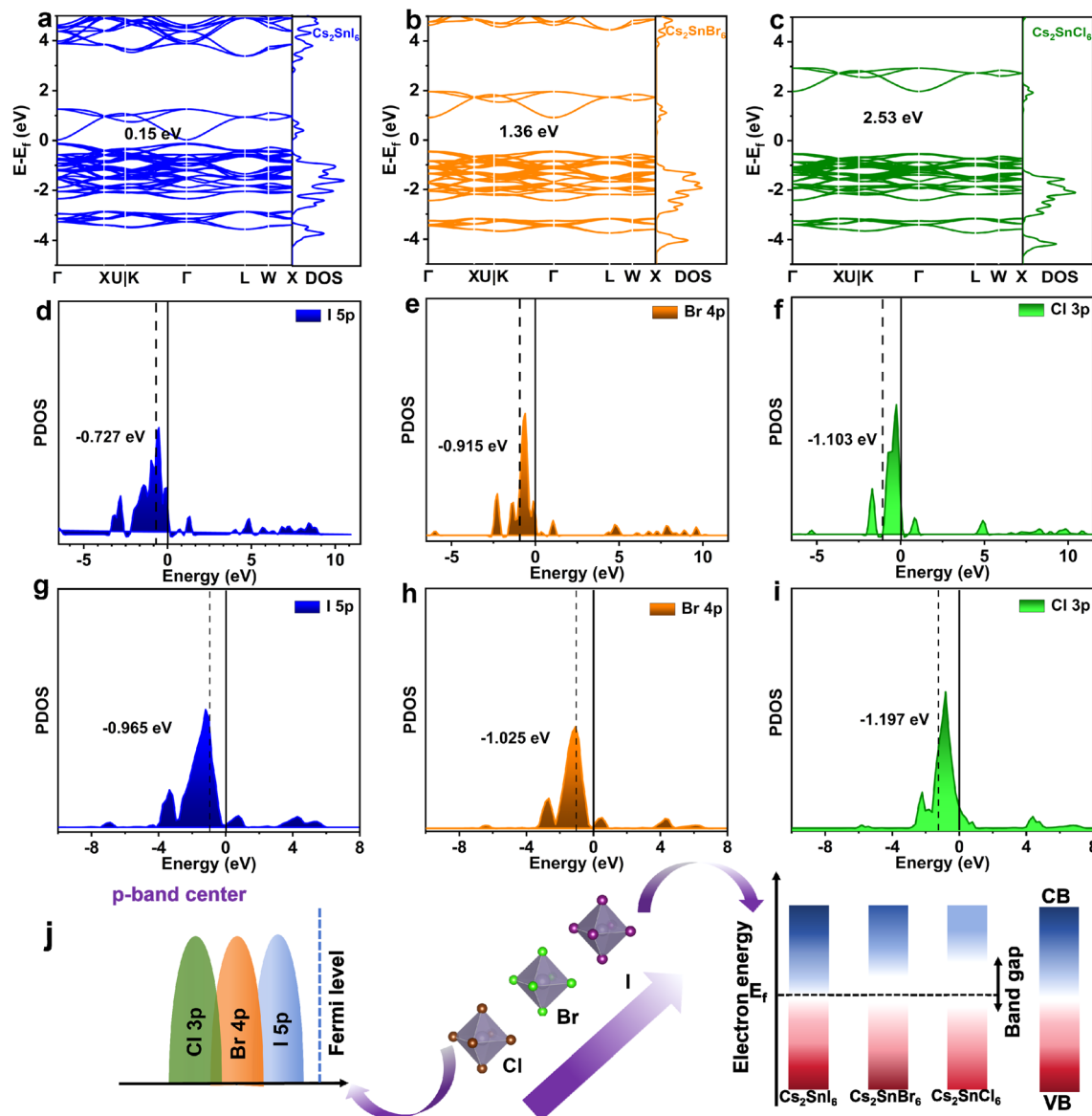
Fig. 1 DFT calculations of \text{Cs}_2\text{SnX}_6 (X = Cl, Br, I): electronic band structures of (a) \text{Cs}_2\text{SnI}_6 , (b) \text{Cs}_2\text{SnBr}_6 , and (c) \text{Cs}_2\text{SnCl}_6 . (d–i) PDOS files of (d and g) I 5p, (e and h) Br 4p, and (f and i) Cl 3p for (d–f) fresh \text{Cs}_2\text{SnX}_6 and (g–i) after adsorbing \text{Li}_2\text{S}_6 . (j) Schematic illustration of the p-band center regulation and electronic band structure of halide anions in \text{Cs}_2\text{SnX}_6 .
