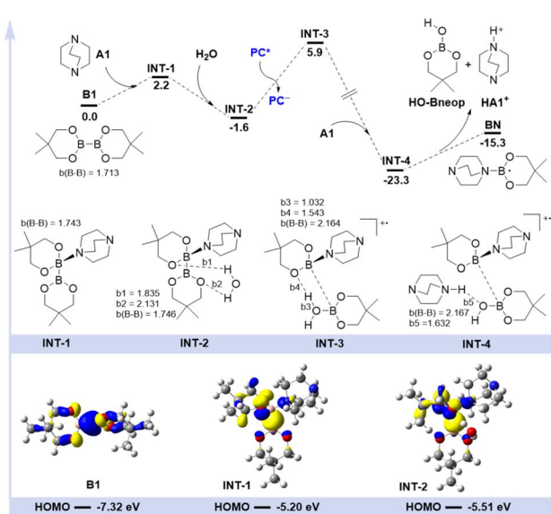
Scheme 3 DFT calculated potential energy surface and frontier molecular orbital analysis for the ligated boryl radical formation process in \text{kcal mol}^{-1} .
