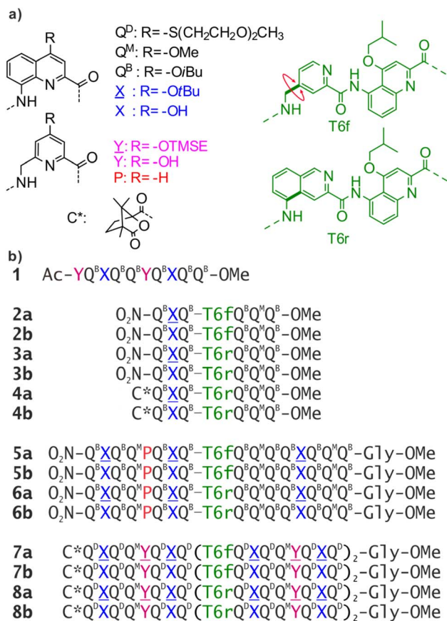
Fig. 1 (a) Structure of Q^D , Q^B , Q^M , X , Y , P , T6f , and T6r monomers as well as N-terminal chiral C^* group. X and Y are the hydroxy protected precursors of X and Y , respectively. TMSE = 2 -trimethylsilylethyl. (b) Oligoamide foldamer sequences. The Gly at the C terminus stands for glycine. In sequences ending with an 8-nitro group, this group replaces the terminal amine.
