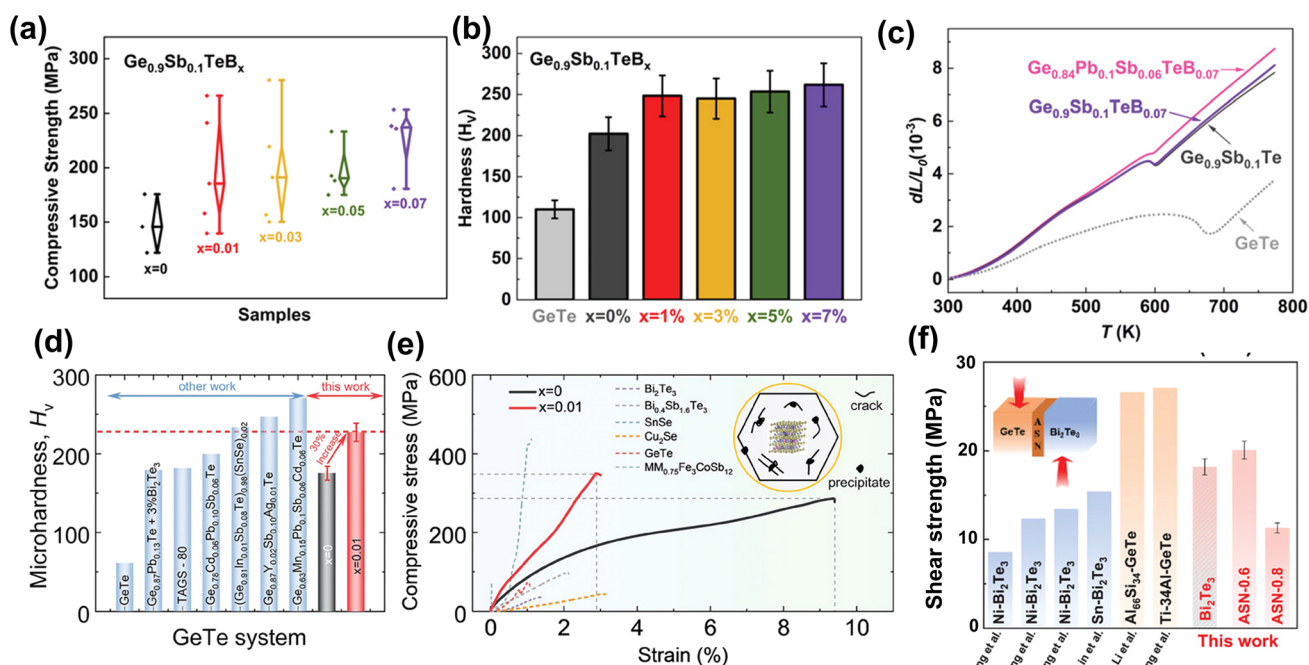
Fig. 24 (a) Compressive strength and (b) Vickers hardness of Ge 0.9 Sb 0.1 Te x . (c) Temperature dependence of relative length variation ( dL/L_0 ). 33 (d) Comparison of room-temperature Vickers microhardness H_v . (e) Comparison of compressive tests of GeTe and some other typical brittle thermoelectric materials. 50 (f) Comparison of the shear strength of the segmented legs and some joints. 190
