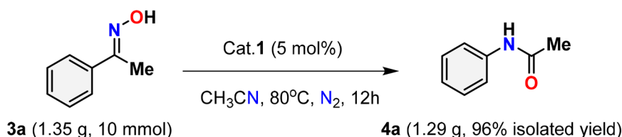
Scheme 4 Gram-scale synthesis of N -phenylacetamide 4a .
