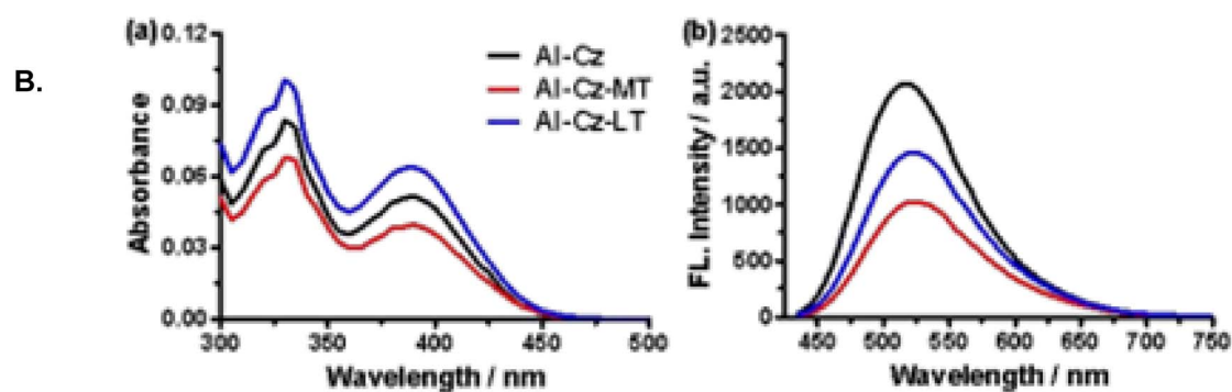
Fig. 13 (A) The synthesis of organelle-specific fluorescent probes 35 and 36 . (B) The absorption and emission spectra of Al-Cz ( 33 ), Al-Cz-MT ( 35 ), and Al-Cz-LT ( 36 ). Reproduced from ref. 42 with permission from American Chemical Society, Copyright © 2023.
