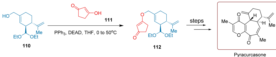
Scheme 46 Dai's synthesis of pyracurasone.
