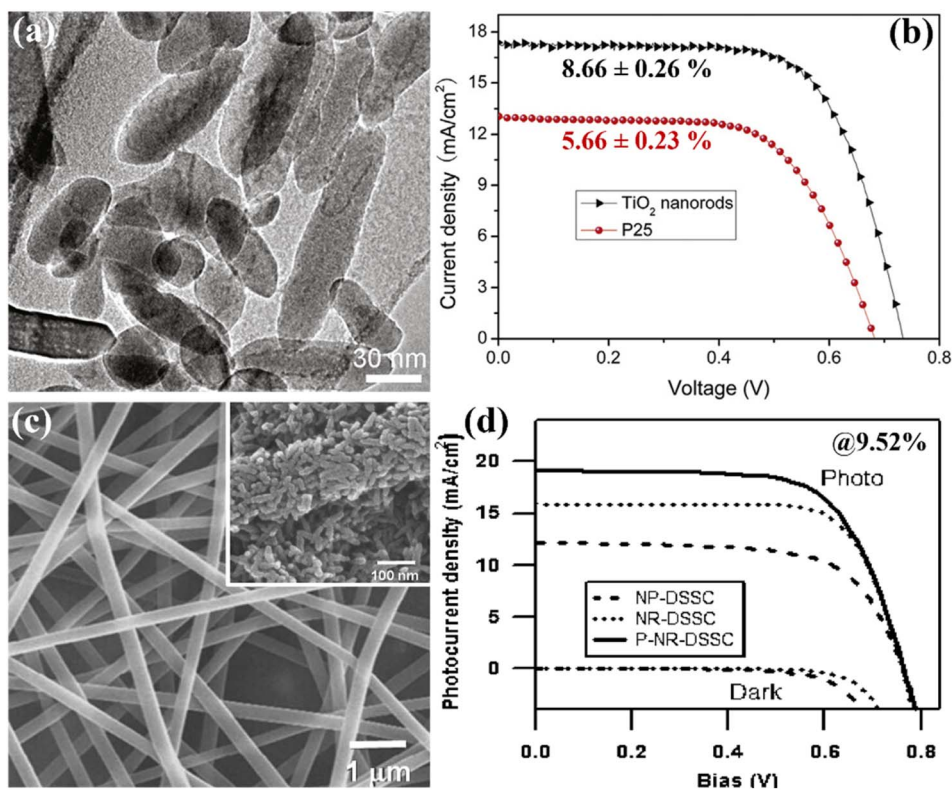
Fig. 13 (a and b) High resolution TEM image of single crystalline anatase \text{TiO}_2 nanorods and the respective DSSC performance with 8.66% PCE, 84 (c and d) typical SEM image of electro-spun \text{TiO}_2 -PVAs nanofibers with heat treated @400 °C SEM image in inset and their consequent performance with PCE of 9.52%. 85
