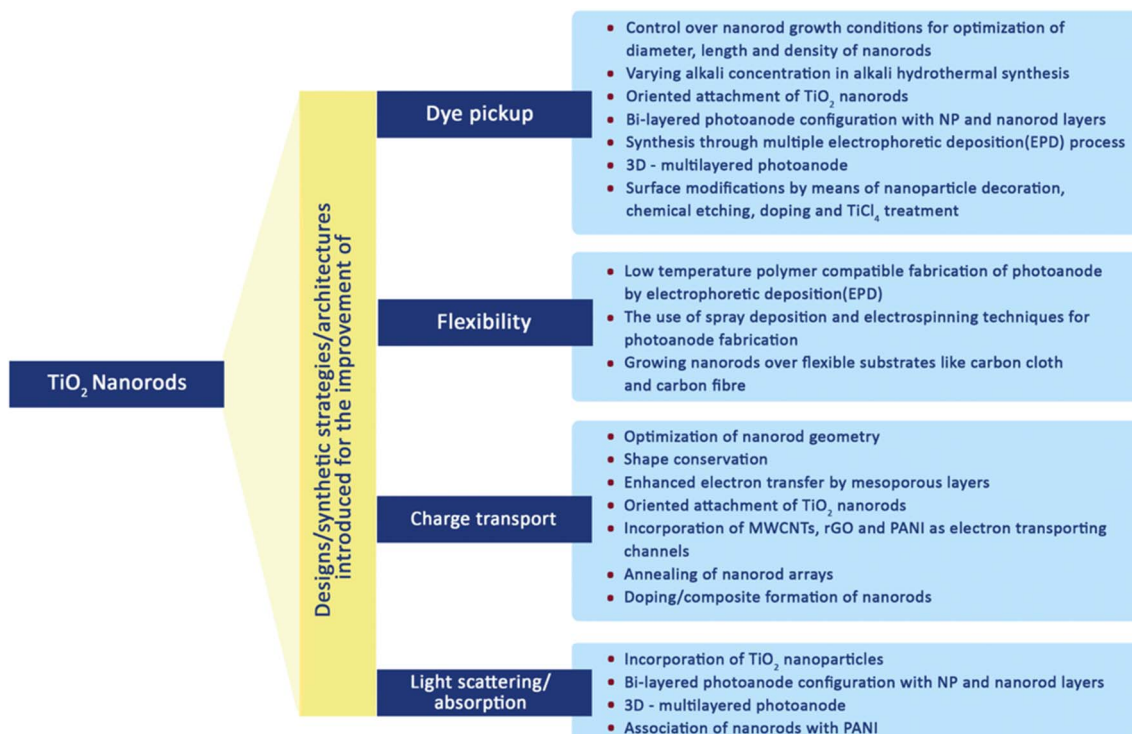
Fig. 12 Various modifications made in \text{TiO}_2 nanorods to improve the DSSCs performance. 70
