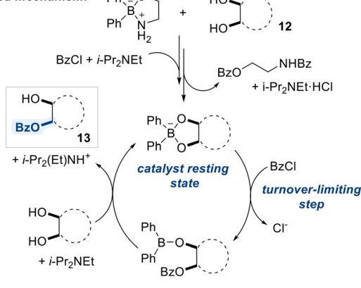
Scheme 9 Borinic acid-catalyzed regioselective acylation of diols.
