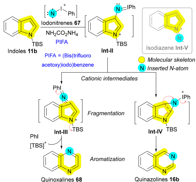
Scheme 8 Nitrogen atom insertion into the main skeleton of indoles leading to ring expansion.
