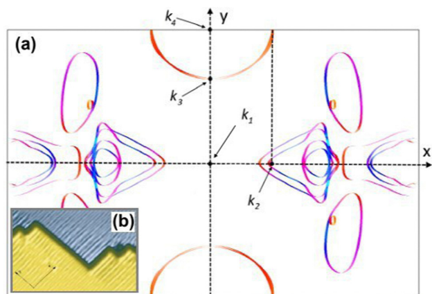
Fig. 13 (a) Unusual Fermi surface section of 24-layer Be(1010) calculated using Quantum Espresso 7.3 100,101 with the SSPP PBEsol Precision v1.3.0 functional 102 and visualised using FermiSurfer. 103 Highlighted k -points: k_2 = 0.64 \text{ \AA}^{-1} , k_3 = 1.33 \text{ \AA}^{-1} , k_4 = 1.75 \text{ \AA}^{-1} . (b) Anisotropic Friedel oscillations due to steps on the surface visible only along the y axis. Reprinted with permission from the work of Hofmann et al. 75
