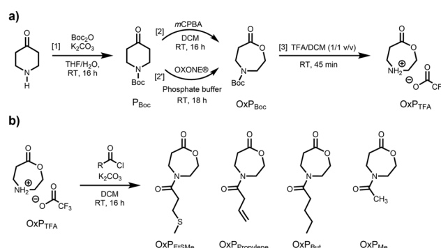
Fig. 1 (a) Three-step synthetic route toward 1,4-oxazepan-7-one trifluoroacetate ( OxP TFA ) starting from 4-piperidone. [1] Boc protection, quantitative yield; [2] Bayer-Villiger ring-expansion, 64%; [2'] oxidation with OXONE®, 80%; [3] Boc-deprotection; 95%. (b) One-step acylation of OxP TFA for the synthesis of four N -acylated-1,4-oxazepan-7-one (OxP) monomers with different side chains and functional groups.
