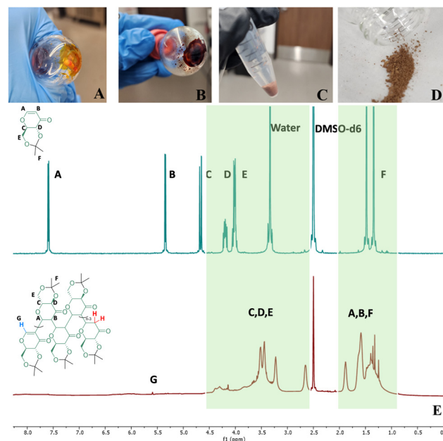
Fig. 1 Synthesis of poly (dimethyl acetal-3-keto-D-glucal) with DBU. Photos of (A) reaction at 1 h, (B) reaction at 16 h, (C) precipitation in water, followed by ether precipitation from DCM, and (D) tan precipitate obtained after drying. The characterization was performed and shown in (E) is the stacked NMR spectra of CAP monomer and poly (dimethyl acetal-3-keto-D-glucal). Note: Stereochemistry not shown for clarity.
