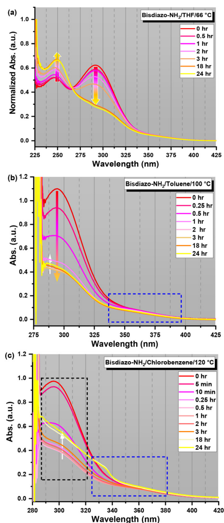
Fig. 3 UV-vis kinetic traces of the polymerization of the bisdiazon-HNH 2 compound in (a) THF as the solvent at 66 °C, (b) toluene at 100 °C and (c) chlorobenzene at 120 °C (concentration = 0.4 mg mL -1 ). UV-vis kinetic rate analysis: kinetic observation of the polymerization of bisdiazon-HNH 2 in different solvent–temperature combinations using eqn (S11) and (S12).†
