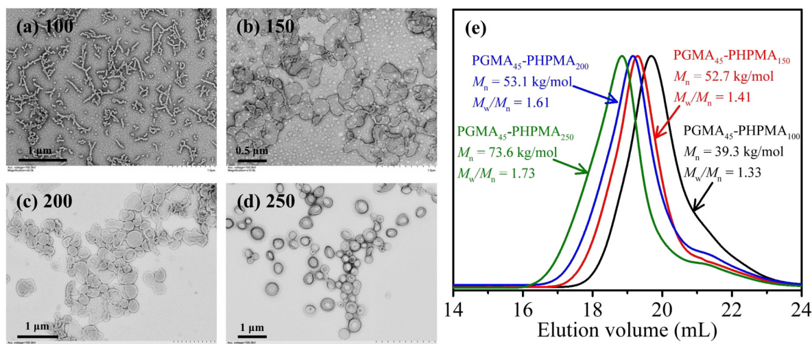
Fig. 2 (a–d) TEM images of block copolymer nanoparticles prepared by photoinitiated RAFT dispersion polymerization of HPMA (15% w/w) in water using \text{PGMA}_{45}\text{-CEPA} with different [\text{HPMA}]/[\text{PGMA}_{45}\text{-CEPA}] ratios. (e) DMF SEC traces of block copolymers synthesized by photoinitiated RAFT dispersion polymerization of HPMA (15% w/w) in water using \text{PGMA}_{45}\text{-CEPA} with different [\text{HPMA}]/[\text{PGMA}_{45}\text{-CEPA}] ratios.
