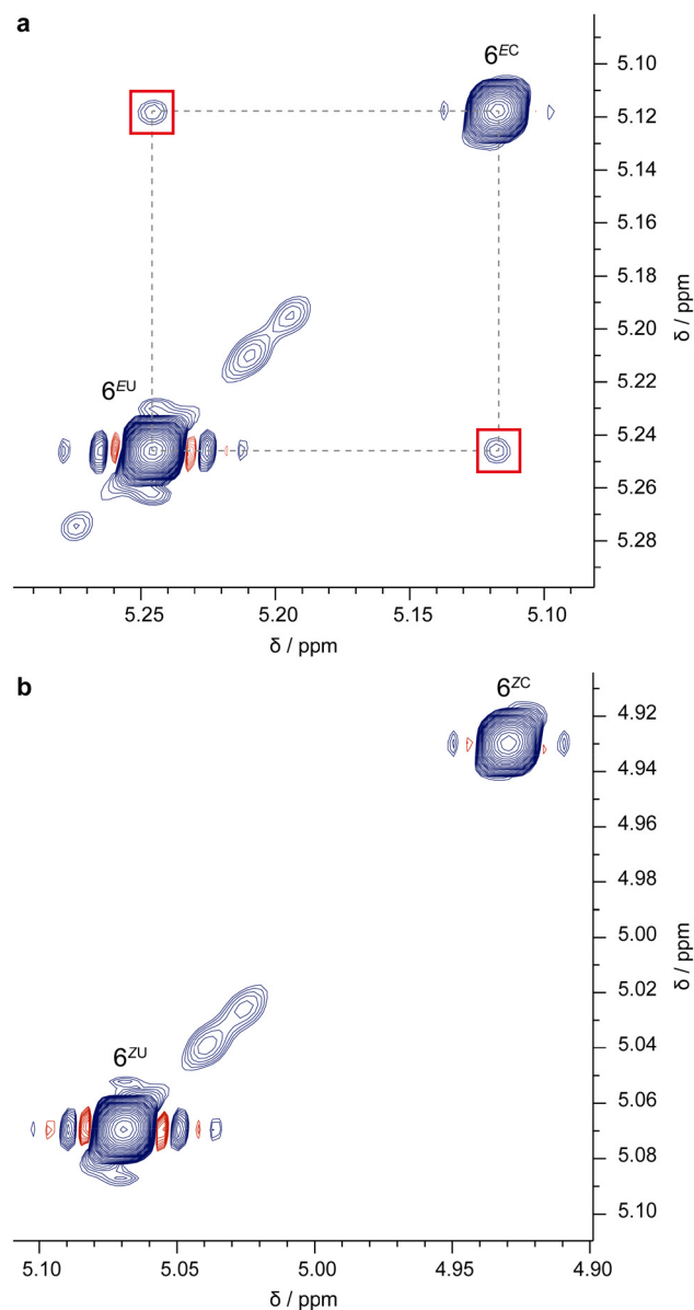
Fig. 5 Partial EXSY NMR ( \text{CD}_3\text{CN} , 500 MHz, 298 K, 1.4 mM, t_{\text{mix}} = 600 \text{ ms} ) spectra of (a) an equimolar mixture of EE\text{-}4\text{H}^+ and 2 , and (b) the same sample after exhaustive irradiation at 365 nm. 6^{EU} and 6^{EC} in (a) indicates the free and complexed EE axle, respectively, whereas 6^{ZU} and 6^{ZC} in (b) denote the free and complexed ZZ axle, respectively.
