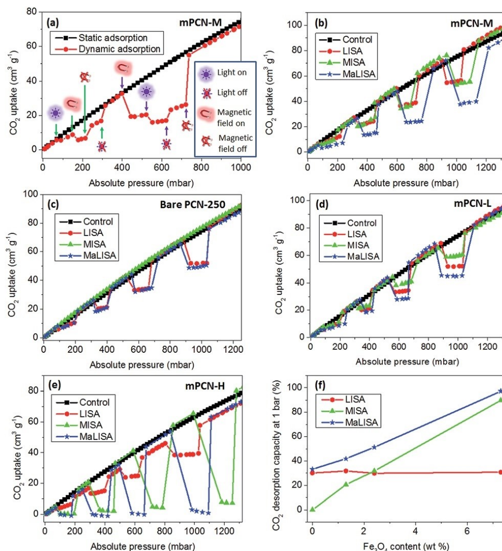
Fig. 11 Two successive typical switching cycles of CO 2 uptake and release in mPCN-M through LISA, MISA and MaLISA processes (a); dynamic switching of CO 2 capture and release in mPCN-M (b), bare PCN-250 (c), mPCN-L (d), and mPCN-H (e) by LISA, MISA and MaLISA processes; (f) shows the CO 2 desorption capacities of mPCNs at 1 bar adapted from the data shown in (b)–(e); all the dynamic CO 2 adsorption profiles were obtained by intermittently exposing the samples to 365 nm UV light (LISA process) and/or an alternating magnetic field of 17.6 mT (MISA process) during the CO 2 adsorption measurement at 298 K. MNP content ranging from 1.3 wt% (mPCN-L), 2.4 wt% (mPCN-M), to 7.3 wt% (mPCN-H). Reproduced from Ref.124 with permission from the Royal Society of Chemistry.
