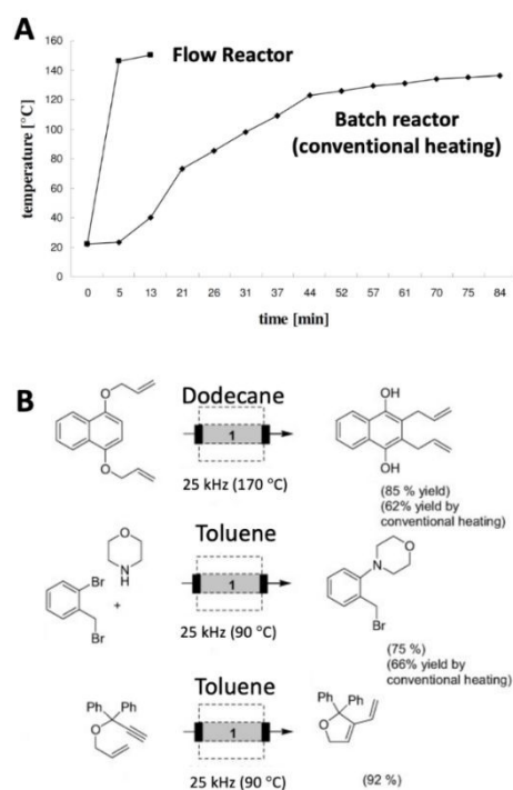
Fig. 8 A) Heating profile of a batch reactor (oil bath with temperature control) in comparison to a flow reactor (inductively heated magnetic nanoparticles, 25 kHz, 340 per mille); B) Selected chemical processes that were successfully catalysed with inductive heating mediated by MNPs. Along, yields of isolated products produced by either conventional heating (batch reactor) and flow reactor (inductively heated) are shown. Adapted with permissions of John Wiley & Sons, Inc. Work from Ceylan, S. et al. 17
