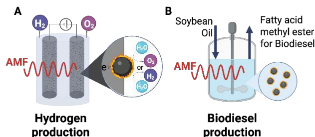
Fig. 10 Use of MH in green fuel production. (A) In hydrogen production, AMFs can activate magnetic catalysts, enhancing water electrolysis by locally increasing reaction temperature and improving electron transfer. (B) In biodiesel production, AMF-induced heating of magnetic nanoparticles accelerates transesterification of oils (e.g., soybean oil) into fatty acid methyl esters, optimizing yield and energy efficiency. Figure created in Biorender.
