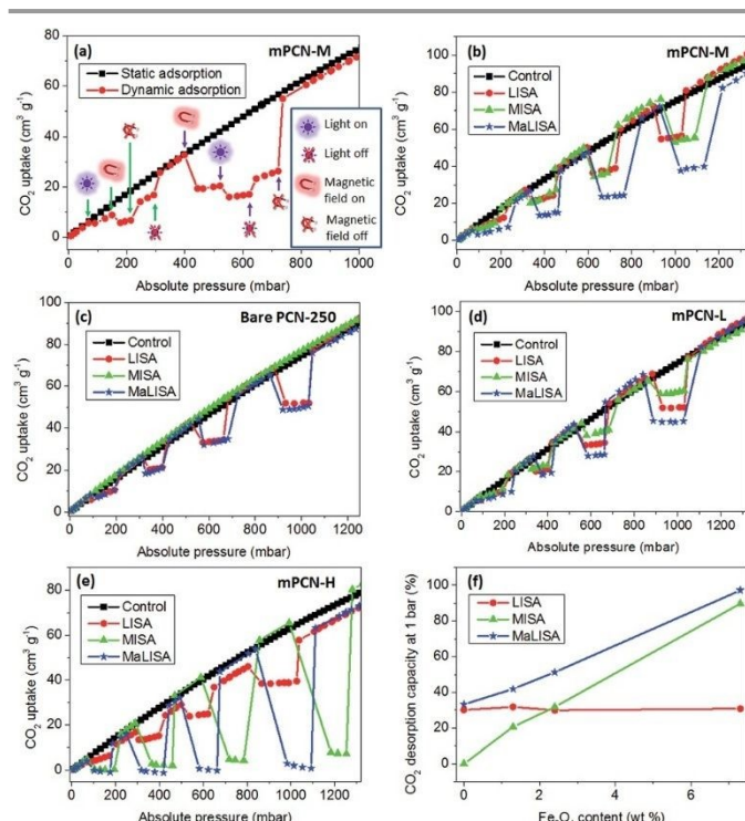
Fig. 11 Successive typical cycles of CO 2 uptake and release using Metal-organic frameworks (MOFs) called PCN-250 (an Iron-based Porous Coordination Network) with embedded magnetic nanoparticles. The magnetic PCN-250 (mPCN) was used with an increasing content of MNPs ( L < M < H ) ranging from 1.3 wt% (mPCN-L), 2.4 wt% (mPCN-M), to 7.3 wt% (mPCN-H). Three excitation approaches were used: LISA (light-induced swing adsorption), MISA (magnetic induction swing adsorption) and MaLISA (a combination of LISA and MISA) processes. (a) Two successive typical switching cycles of CO 2 uptake and release in mPCN-M through LISA, MISA and MaLISA processes. (b, c and d and e) dynamic switching of CO 2 capture and release in mPCN-M (b), bare PCN-250 (c), mPCN-L (d), and mPCN-H (e) by LISA, MISA and MaLISA processes. (f) CO 2 desorption capacities of mPCNs at 1 bar adapted from the data shown in (b)–(e). All the dynamic CO 2 adsorption profiles were obtained by intermittently exposing the samples to 365 nm UV light (LISA process) and/or an alternating magnetic field of 17.6 mT and 279 kHz (MISA process) during the CO 2 adsorption measurement at 298 K. Reproduced from Ref. 162 with permission from the Royal Society of Chemistry.
