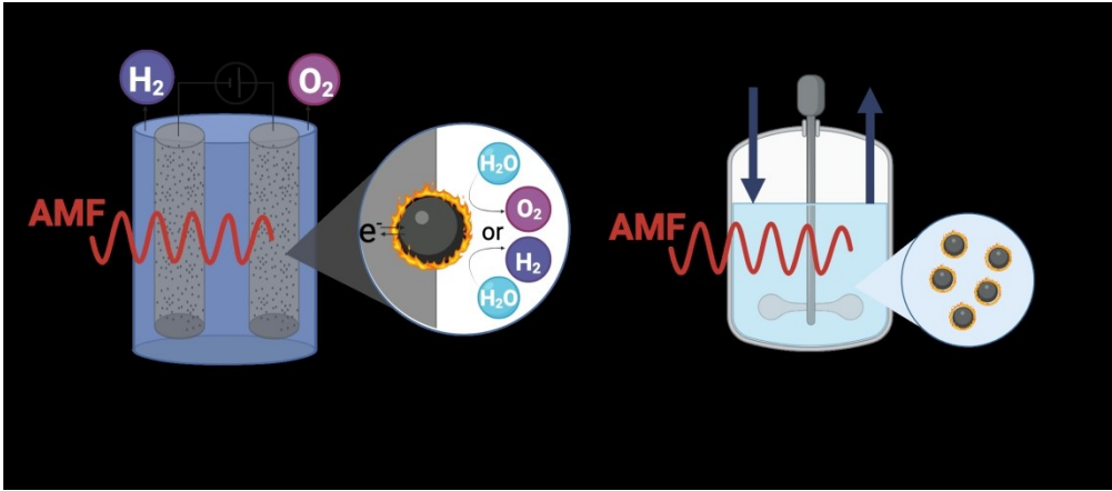
Figure 10. Use of magnetic hyperthermia in green fuel production. (A) In hydrogen production, AMFs can activate magnetic catalysts, enhancing water electrolysis by locally increasing reaction temperature and improving electron transfer. (B) In biodiesel production, AMF-induced heating of magnetic nanoparticles accelerates transesterification of oils (e.g., soybean oil) into fatty acid methyl esters, optimizing yield and energy efficiency.
