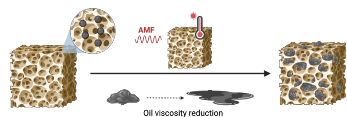
Fig. 14 Schematic illustration of the design required for Enhanced Oil Recovery (EOR) methods using MNPs (also the so-called "ferrimagnetic sponge"). MH leads to efficient clean-up of viscous crude oil. Figure created in Biorender.
