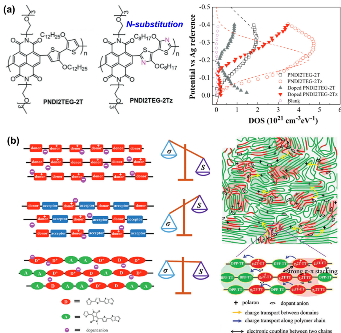
Fig. 4 (a) \text{sp}^2 N -substitution in the donor moiety makes the DOS of the donor–acceptor copolymer narrower (degenerate), which is ideal for maintaining a high \sigma and S 34 (reproduced with permission, Copyright 2018, Wiley-VCH). (b) Polymers with only donors have a high \sigma and low S , polymers with an alternate sequence of donors and acceptors have a high S due to interchain energetic disorder but low \sigma , whereas polymers with a random sequence of donors and acceptors have both high S and \sigma 21 (reproduced with permission, copyright 2020, Wiley-VCH).
