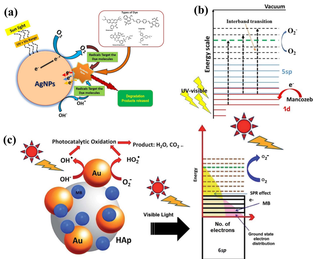
Fig. 2 (a) Schematic diagram of photocatalytic degradation of dyes. 13 (b) Band structure of Ag NPs and its photocatalytic mechanism. 39 (c) Mechanism of waste removal utilizing plasmonic Au NPs based photocatalysts. 58 Reproduced from ref. 58 with permission from the Royal Society of Chemistry. Copyright © 2020 Elsevier B.V. All rights reserved.
