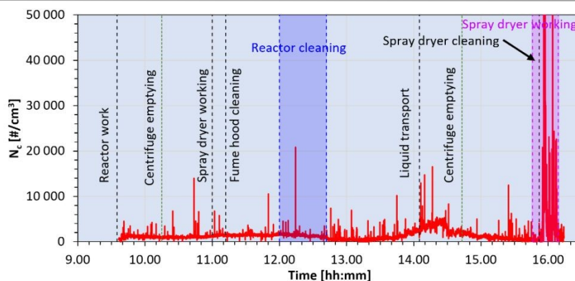
Fig. 4 Particle number concentrations ( d_p = 10\text{--}700 \text{ nm} , DISCmini) at the worker's breathing zone during GO production over a 7-hour work shift (Scenario 6).
