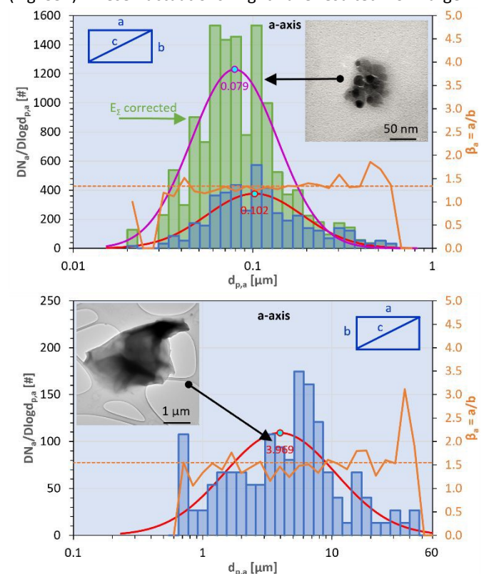
Fig. 6 Number size distribution of 0.02–0.55 μm ( n=252 , above) and 0.55–50 μm ( n=118 , below) particles for the a-axis. The blue histogram presents the number of counted particles, while the green histogram shows the distribution corrected for collection efficiency ( E_z ). 54,55 Red and pink curves depict fitted lognormal distributions. The orange curve shows the aspect ratio ( \beta=a/b ), with the dotted orange line indicating the average aspect ratio. Examples of particle morphology are displayed as TEM images.
