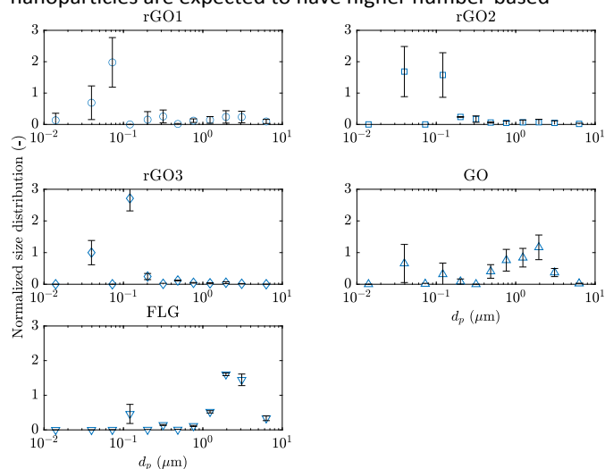
Fig. 2 Normalised number size distributions f_n(d_{p,i}) , for dustiness-tested GRMs, showing the mean and standard deviation for each ELPI stage. 60 Data points near 0.07 \mu\text{m} for rGO2, rGO3, and GO are suspected outliers, likely due to a single ELPI stage becoming filled or clogged with GRM.
