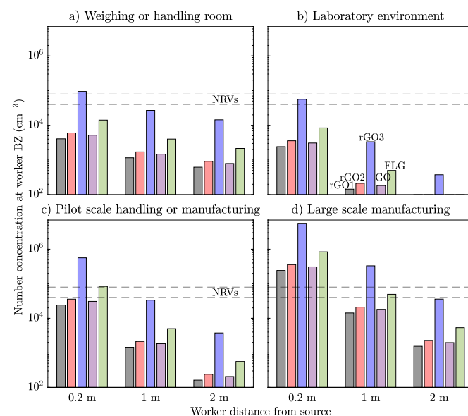
Fig. 7 Modelled number concentrations at the worker's breathing zone, shown as bars from left to right, for rGO1 (black), rGO2 (red), rGO3 (blue), GO (purple) and FLG (green). Laboratory-scale powder handling in a) weighing room ( 4 \times 4 \times 2.5\text{ m}^3 , 0.5\text{ h}^{-1} ) and b) laboratory environment ( 9 \times 6 \times 3\text{ m}^3 , 18\text{ h}^{-1} ); c) pilot-scale (10-fold) handling or manufacturing in a similar laboratory environment; and d) industrial-scale (100-fold) manufacturing in a factory hall ( 30 \times 20 \times 7\text{ m}^3 , 18\text{ h}^{-1} ). The nano reference values (NRVs) for 8 h and 15 min exposures ( 40,000 and 80,000\text{ cm}^{-3} ) are indicated with horizontal dashed lines. Note the logarithmic y-axis.
