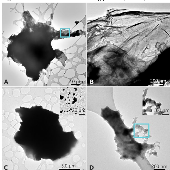
Fig. 5 TEM images of particles collected at the worker's breathing zone during the spray dryer cleaning task in GO production (Scenario 6). A) GO particle; B) fine structural detail; C) large GO particles; and D) an agglomerate composed of nanoscale primary particles.
