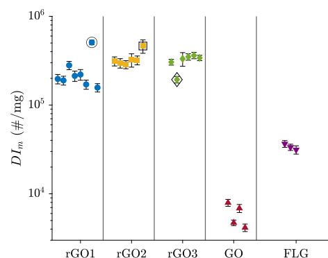
Fig. 1 Number-based dustiness indices for five GRMs from individual dustiness tests ( n=27 ), based on UCPC data ( d_p = 2.5 \text{ nm} - 1 \text{ }\mu\text{m} ). Error bars indicate the limits from propagation of uncertainty (maximal error). Outliers, encircled on the plot, likely result from measurement inconsistencies, such as partial clogging of sampling lines or the cyclone with GRM, affecting sampling flows or releasing GRM.
