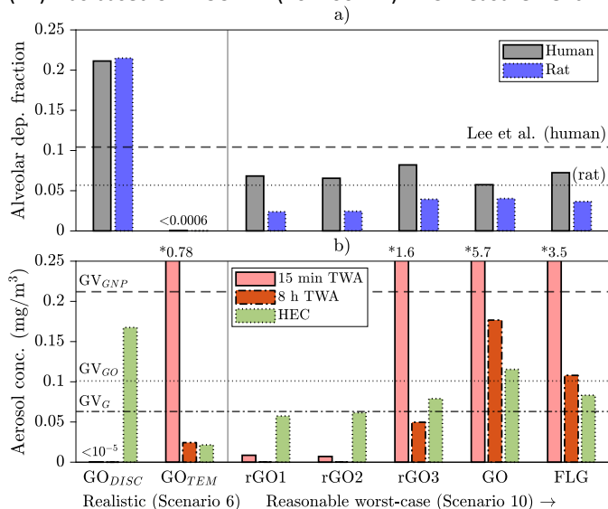
Fig. 8 a) Modelled alveolar deposition fractions in human and rat respiratory tracts for seven MPPD simulations covering multiple GRMs. Horizontal lines represent comparable values calculated for GO by Lee et al. 65 b) Exposure concentrations (red) as 15 min and 8 h time weighted averages (TWA) for a real-world exposure (Scenario 6) based on workplace sampling with DISCmini ( GO_{DISC} ) and electron microscopy ( GO_{TEM} ). Reasonable worst-case exposure estimates (Scenario 10) are based on exposure modelling. Calculated human equivalent concentrations (HEC, green) are based on the no-observed adverse-effect concentration in rats. 66 Horizontal lines indicate guidance values for graphene nanoplatelets ( GV_{GNP} , 74 GV_{G^{75}} ) and GO ( GV_{GO} ) 75 extracted from the literature.
