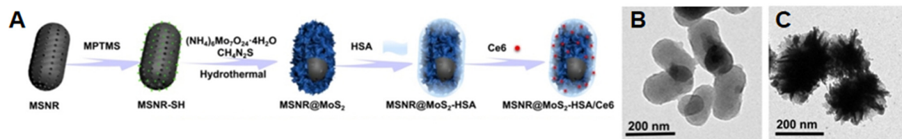
Fig. 9 Preparation and characterization of TMD-based ternary and multinary compounds. (A) Schematic illustration of the preparation of \text{MSNR@MoS}_2\text{-HSA/Ce6} . TEM images of (B) MSNR and (C) \text{MSNR@MoS}_2 . 33 Reproduced with permission from ref. 33. Copyright 2019 Ivyspring International Publisher.
