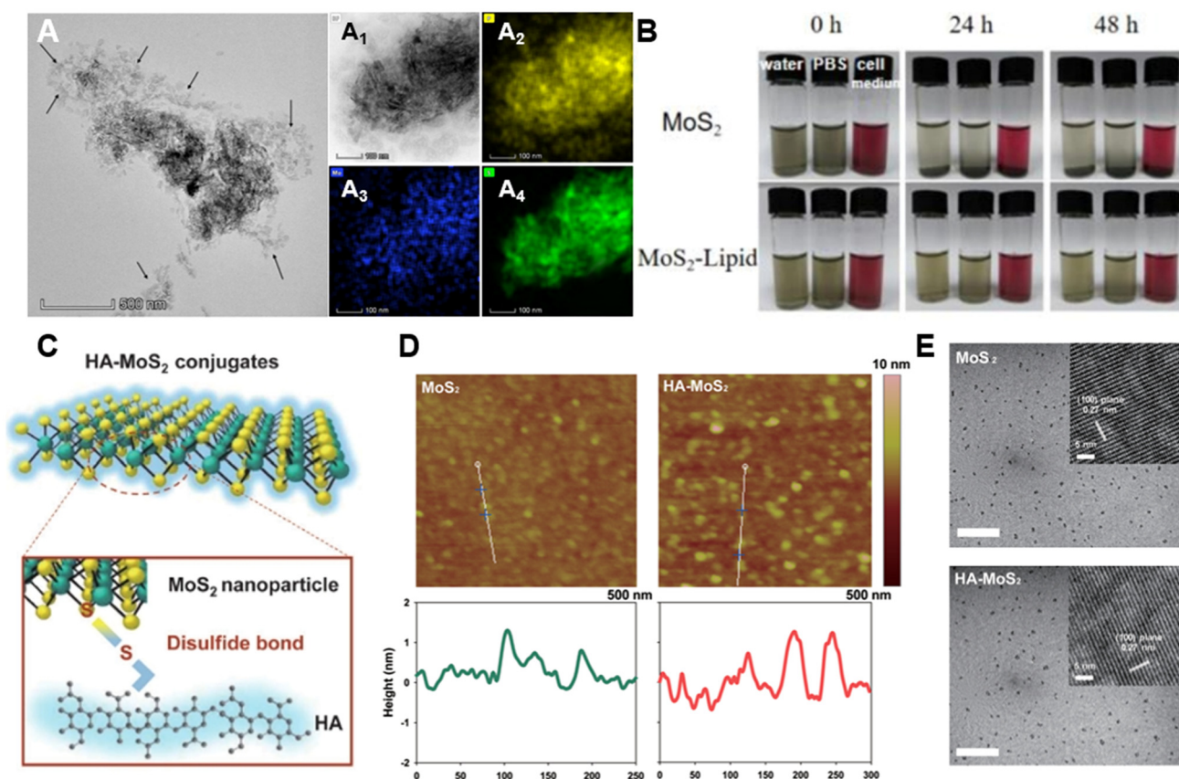
Fig. 4 Preparation and characterization of TMD-organic material composites. (A) Typical TEM image of the \text{MoS}_2 -lipid. A_1 – A_4 are bright-field scanning transmission electron microscopy (BF-STEM) images of the \text{MoS}_2 -lipid and the corresponding energy dispersive X-ray (EDX) element mappings of P, S, and Mo, respectively. (B) Photographs of \text{MoS}_2 (upper) and \text{MoS}_2 -lipid (bottom) incubated in water, PBS and cell culture medium (containing 10% fetal bovine serum) for 24 hours and 48 hours. 74 Reproduced with permission from ref. 74. Copyright 2020 Elsevier. (C) Scheme of HA- \text{MoS}_2 conjugates. (D) AFM images (upper) and the corresponding height profiles (bottom) of \text{MoS}_2 (left) and HA- \text{MoS}_2 (right). (E) TEM images of \text{MoS}_2 (top) and HA- \text{MoS}_2 (bottom) (scale bar = 500 nm). Insets: high-resolution TEM (HRTEM) images of \text{MoS}_2 and HA- \text{MoS}_2 . 36 Reproduced with permission from ref. 36. Copyright 2019 Wiley-VCH.
