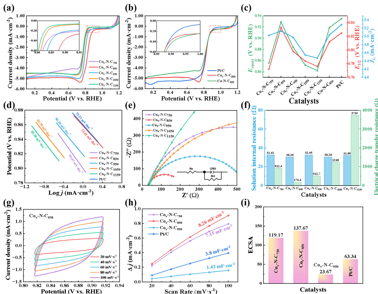
Fig. 4 (a and b) LSV curves in O 2 -saturated 0.1 M KOH solution (scanning rate: 10 mV s -1 ; rotation speed: 1600 rpm). (c) Onset potential, half-wave potential and limiting current density of various catalysts. (d) Tafel plots of the corresponding polarization curves, (e) EIS Nyquist plots for Co-N-C catalysts, and (f) solution internal resistance and charge transfer internal resistance of various catalysts. (g) Cyclic voltammograms curves of the Co v -N-C 850 in N 2 -saturated 0.1 M KOH solution at different scan rates from 20 to 100 mV s -1 , (h) plots of current density against scan rates, and (i) the electrochemically active surface area (ECSA) for Co v -N-C 750 , Co v -N-C 850 , Co v -N-C 950 , and commercially available Pt/C, respectively.
