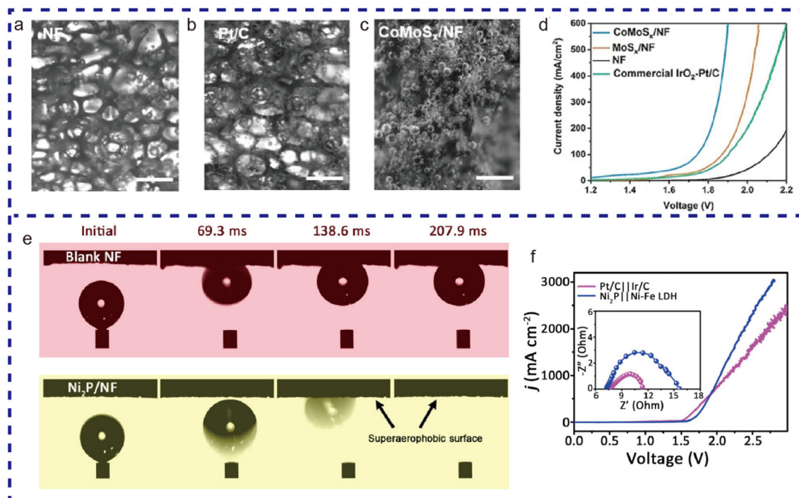
Fig. 4 Digital images showing bubbles released from (a) NF, (b) Pt/C, and (c) \text{CoMoS}_x/\text{NF} during HER at a current density of 200 \text{ mA cm}^{-2} . Scale bars are 0.5 mm. (d) LSV for \text{CoMoS}_x/\text{NF} , \text{MoS}_x/\text{NF} , \text{IrO}_2\text{-Pt/C} , and NF electrodes at a scan rate of 5 \text{ mV s}^{-1} . Reproduced from ref. 87 with permission from Wiley, copyright 2019. (e) Digital images of hydrogen bubbles on NF and \text{Ni}_2\text{P}/\text{NF} . (f) LSV of the catalysts at a scan rate of 10 \text{ mV s}^{-1} , with the inset showing EIS Nyquist plots of the catalysts at 1.7 V. Reproduced from ref. 101 with permission from ACS, copyright 2019.
