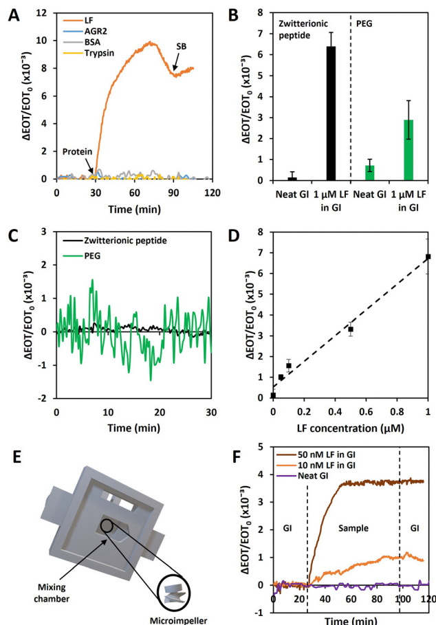
Fig. 4 Biosensor performance: (A) real-time relative EOT changes upon introduction of the target protein LF (90 \mu g mL^{-1} , equivalent to 1 \mu M ) and other non-target proteins (AGR2, BSA and trypsin) at a similar concentration in buffer. (B) Net relative EOT changes in response to the LF-spiked GI fluid (1 \mu M ) comparing the zwitterionic peptide-modified aptasensor with the PEG-passivated biosensor. (C) Baseline comparison in the neat GI fluid. (D) LF binding curve in the GI fluid over a concentration range of 0.05 to 1 \mu M ( n = 3 ). (E) Illustration of the micro-impeller system, consisting of a mixing chamber for the impeller and a measurement zone with a height of 1 mm. (F) Characteristic real-time EOT changes for the micro-impeller system upon introduction of the LF-spiked GI sample at concentrations of 10 and 50 nM LF.
