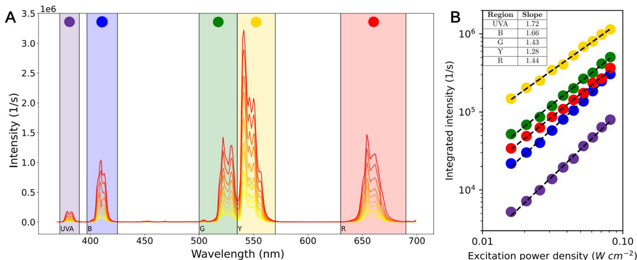
Fig. 3 \beta – NaYF 4 :Yb 3+ , Er 3+ UNCP power dependent spectrum. (A) Emission spectra under CW 976 nm excitation for different incident power densities, ranging from 16 mW cm -2 to 80 mW cm -2 . From left to right, spectral regions labeled at the bottom of the figure named UVA, B, G, Y and R are highlighted. (B) Log–Log plot of the integrated intensity measurements for each of the spectral regions highlighted in (A). An inset table shows the slopes of a linear least squares fit of the data.
