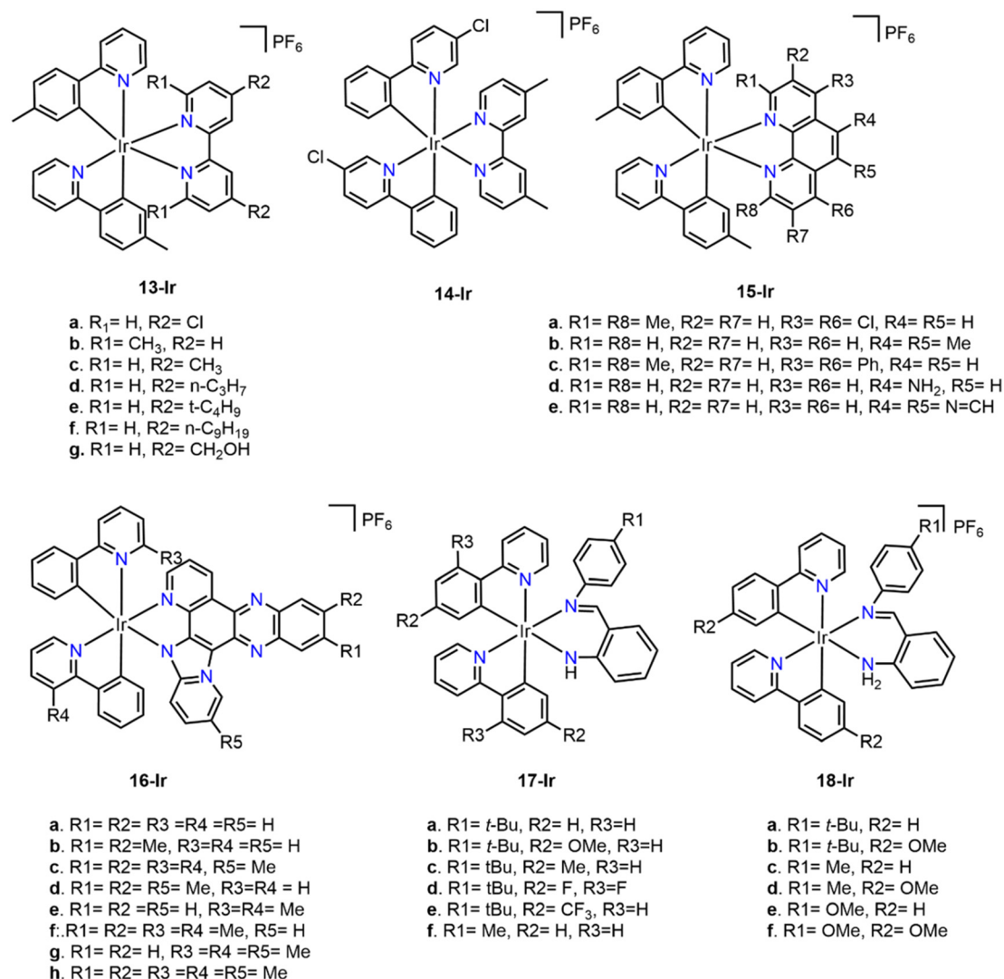
Fig. 36 Ir(III) cyclometalated compounds ( 13-Ir – 18-Ir ) used as potential anticancer agents.
