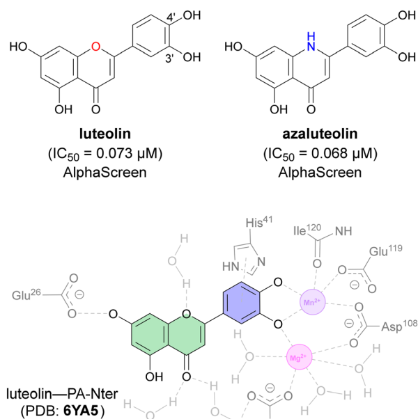
Fig. 1 Flavonoid inhibitors of influenza endonuclease and graphical illustration of the binding mode of luteolin in the PA-Nter active site.
