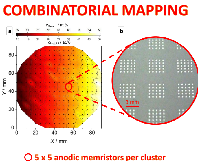
Figure 9: (a) Example of an EDX mapping for a combinatorial library created by alloying 2 valve metals (b) an image of a finished anodic library.
