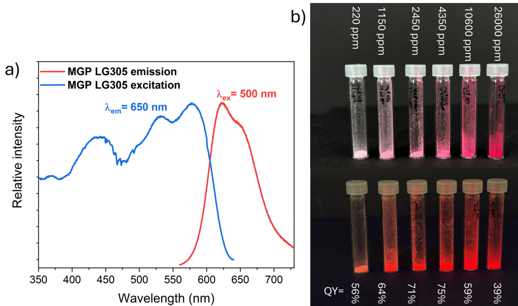
Fig. 10 (a) Emission and excitation spectra of MGP LG305 (1150 ppm LG305) at an excitation wavelength of 500 nm and an emission wavelength of 650 nm, (b) image of MGP LG305 with varying dye concentrations (220–26 000 ppm) under natural light (top) and 450 nm light (bottom), along with their respective quantum yields (QY).
