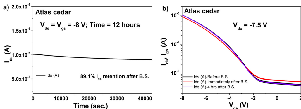
Fig. 16 OFET with Atlas cedar resin and pentacene semiconductor evaluated for bias stress stability: (a) bias stress measurement curve after applying constant voltages to the OFET device, V_{\text{ds}} = V_{\text{gs}} = -8 V for 12 h. (b) Recovery of the transistor characteristics after the bias stress measurements.
