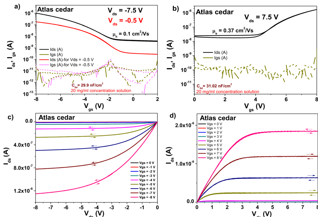
Fig. 15 Transistor measurements of Atlas cedar resin on 10 V anodized aluminum gate electrode ( i.e. , \sim 16\text{--}17 nm thick aluminum oxide, \text{Al}_2\text{O}_3 ) with pentacene and \text{C}_{60} as the organic semiconductor: (a) transfer curve of the OFET using pentacene as organic semiconductor. (b) Transfer curve of the OFET using \text{C}_{60} as the organic semiconductor. (c) Output curve of the OFET using pentacene as the organic semiconductor. (d) Output curve using \text{C}_{60} as the organic semiconductor.
