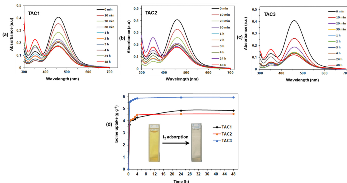
Fig. 12 UV-Vis absorption spectra of an aqueous solution of iodine ( 1 \text{ mM} ) upon adding TAC1 (a), TAC2 (b) and TAC3 (c). Maximum \text{I}_2 adsorption capacity measurements for all three copolymers TAC1–3 (d) (inset: images showing the color change of aqueous \text{I}_2 solutions before and after adsorption by TACs ).
