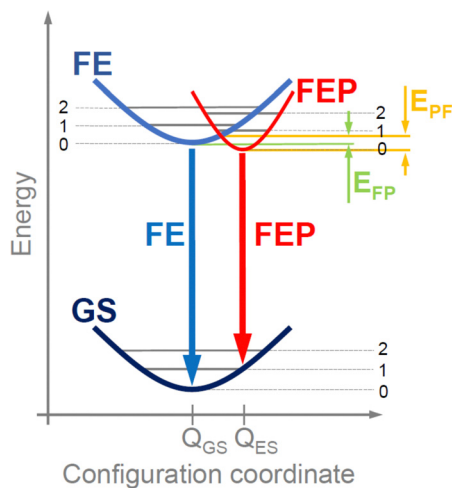
Fig. 2 Configuration diagram for free exciton and FE-polaron transition in EA 2 PbI 4 .
