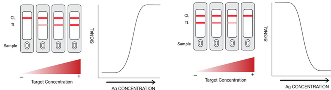
Fig. 1 Schematic representation of LFA signal outputs. (A) Sandwich format: an increase in target analyte concentration leads to a higher intensity of the test line (TL), resulting in a positive correlation between analyte concentration and signal intensity. (B) Competitive format: an increase in target analyte concentration results in a reduction of signal intensity on the TL, demonstrating an inverse correlation between analyte concentration and signal intensity.
