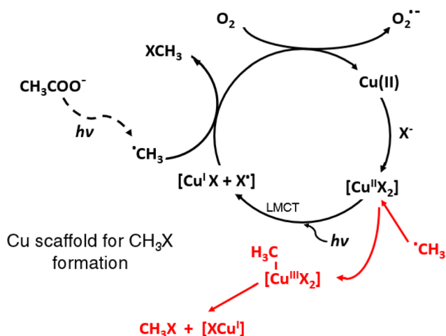
Fig. 1 TM-assisted PVG of halogens using added Cu(II) as an example of aquo-metal halide complex formation followed by (i) \cdot\text{CH}_3 capture of halide atom ( \text{X}' ) formed by a LMCT process or (ii, shown in red) oxidative addition of \cdot\text{CH}_3 to \text{CuX}_2 complex followed by reductive elimination of \text{CH}_3\text{X} and subsequent catalytic re-oxidation of Cu(I) by dissolved oxygen or other oxidants in the system.
