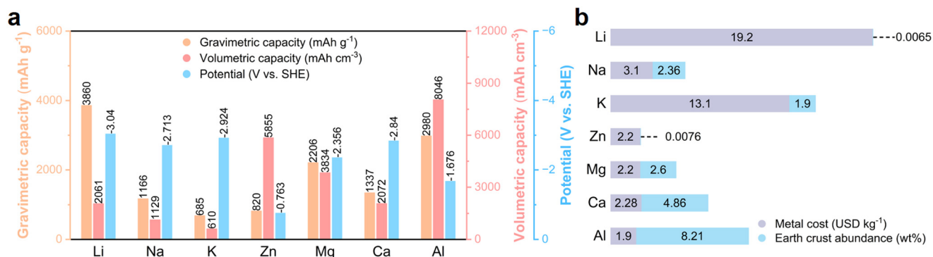
Fig. 1 Advantages of Al as a battery anode. (a) Comparison of theoretical specific capacities and standard electrochemical reduction potentials of different metal anodes. (b) Abundance of different metal elements in the Earth's crust and the cost of metal anodes. Reprinted with permission. 16 Copyright 2021, WILEY-VCH VERLAG GMBH.
