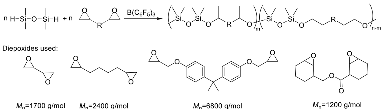
Fig. 11 Polycondensation of diepoxides and hydrosilanes catalyzed by \text{B(C}_6\text{F}_5)_3 . 36
