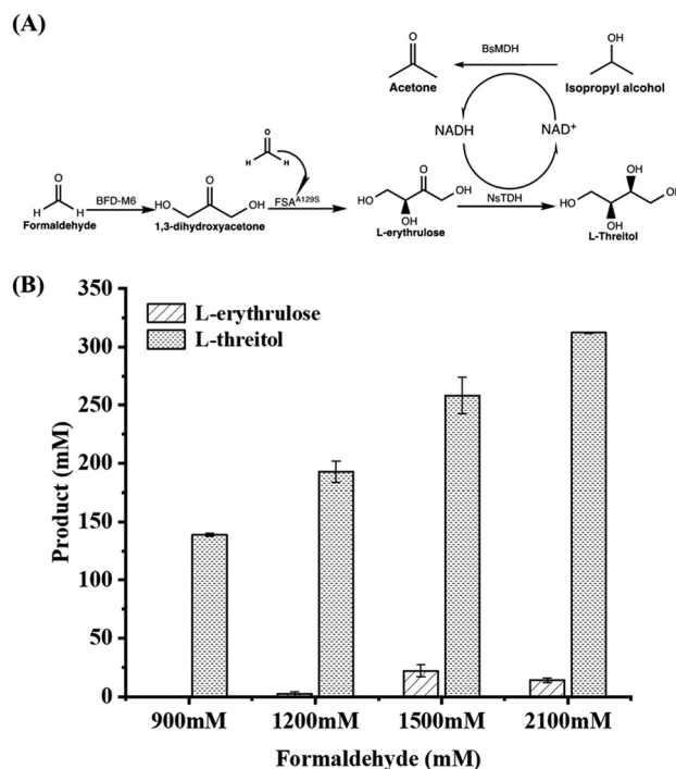
Fig. 6 One-pot two-step synthesis of L-threitol from formaldehyde using the BsMDH/isopropanol system for NADH regeneration. (A) The reaction route for L-threitol synthesis using the BsMDH/isopropanol system for NADH regeneration. (B) The yield of L-threitol at different concentrations of formaldehyde. To produce L-erythrulose, a 750 \mu L standard reaction mixture with phosphate buffer (50 mM potassium phosphate, 5 mM \text{MgSO}_4 , pH 7.4) containing 900, 1200, 1500, or 2100 mM formaldehyde, 0.33 mM \text{FSA}^{\text{A129S}} and 0.13 mM formolase _{\text{BFD-M6}} was used in the first step. The reactions were carried out at 30 ^\circ\text{C} with shaking at 1000 rpm in a 1.5 mL microcentrifuge tube for 8 h. Subsequently, a 1 mL reaction mixture containing 750 \mu L of the first-step solution, 2 mM NADH, 0.11 mM NsTDH, 0.14 mM BsMDH and 170, 220, 280, or 380 mM isopropanol in potassium phosphate buffer was prepared and used in the second step, which was carried out for 12 h.
