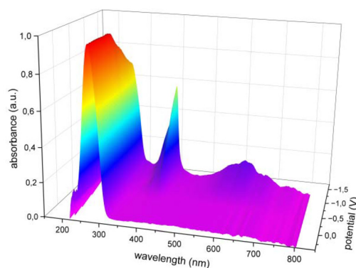
Fig. 2 Spectroelectrochemical measurements of MVCl_2 illustrating the appearance of MV^{\bullet+} in TFE.
